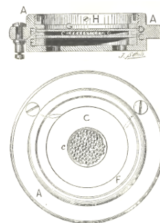
FIG. 66. — Microphone Berthon.
