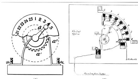
Fig 2-Dial arrangement (a) and switching elements (b) for one subscriber's line illustrated in the Connolly and McTighe patent of 1879 . Similar switching equipment, mounted on a common shaft, was provided for each line of the exchange.
