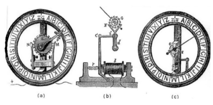
Fig 2-Dial arrangement (a) and switching elements (b) for one subscriber's line illustrated in the Connolly and McTighe patent of 1879 . Similar switching equipment, mounted on a common shaft, was provided for each line of the exchange.
