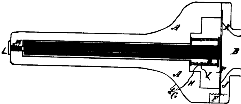
Fig. 1. Section of Telephone.
